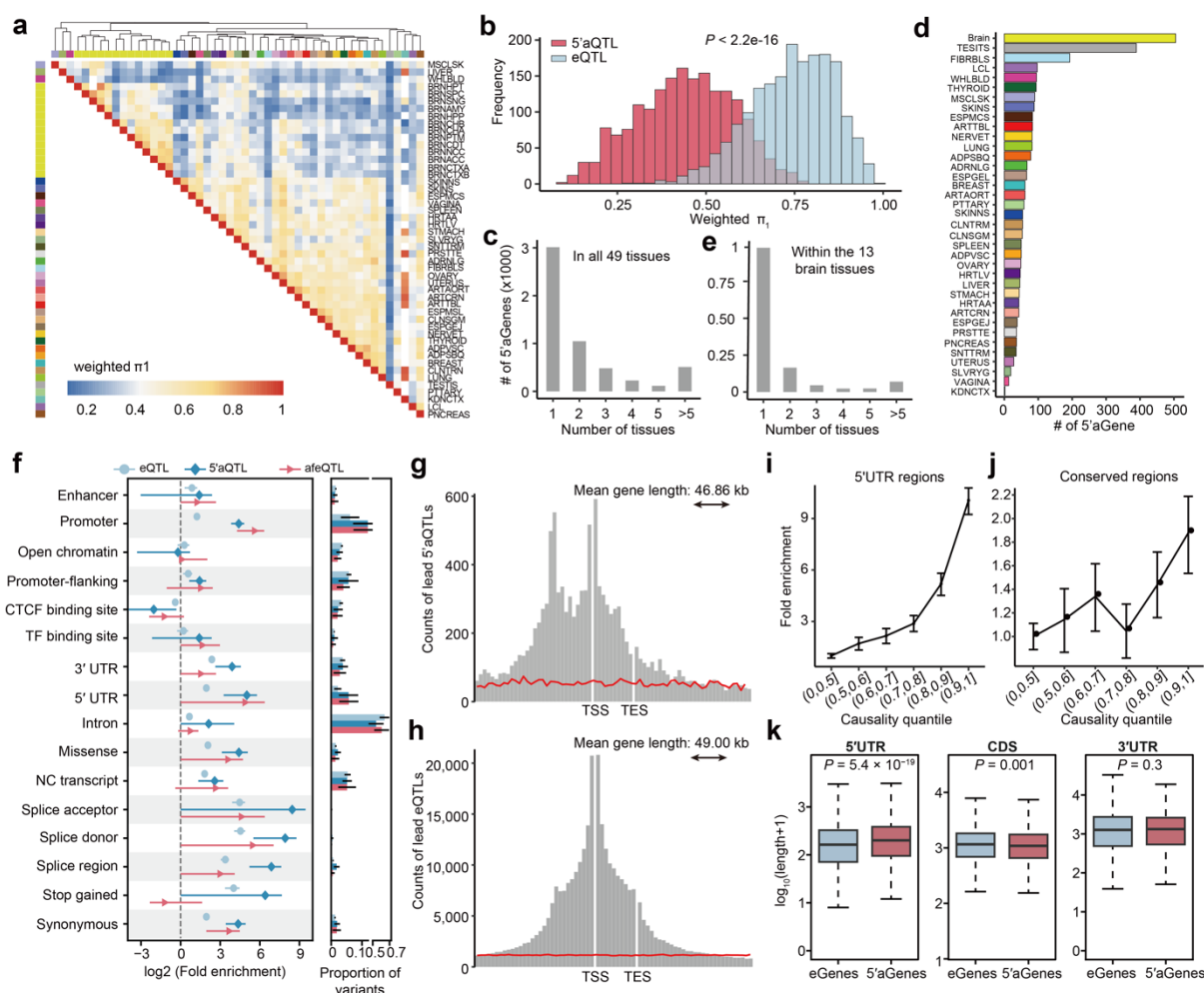
Fig. 2. Tissue-specific 5'aQTLs and distinct genetic variation beyond eQTLs. a , Heatmap shows the sharing relationships between tissues as estimated by weighted \pi_1 metric. The rows of the heatmap present the GTEx tissues (discovery tissues) and tissues order was determined by the method hclust with default settings in R basic package, and the tissues order in columns (replicate tissues) were the same as rows. Missing values were filled with grey. The diagonal presents self-comparison, and the value was assigned as 1 by definition. The color of each cell in the heatmap depend on weighted \pi_1 value. b , The frequency of weighted \pi_1 for pairwise 5'aQTL and eQTL sharing across tissues. P value was obtained from Wilcoxon rank-sum test. c , Number of shared tissues for all 5'aGene across 49 tissues. d , Barplot shows the number of tissue-specific 5'aGene in each of the 49 tissues. e , Number of shared tissues for all 5'aGene across the 13 brain tissues. f , The proportion and enrichment of 5'aQTLs, eQTLs and afeQTLs under different annotations. Fold enrichment was shown as mean (dot) \pm standard deviation ( \log_2 scaled, error bar) across 49 tissues. The error bars in the right panel indicate standard deviation of the proportion of variants across 49 tissues. g-h ,
