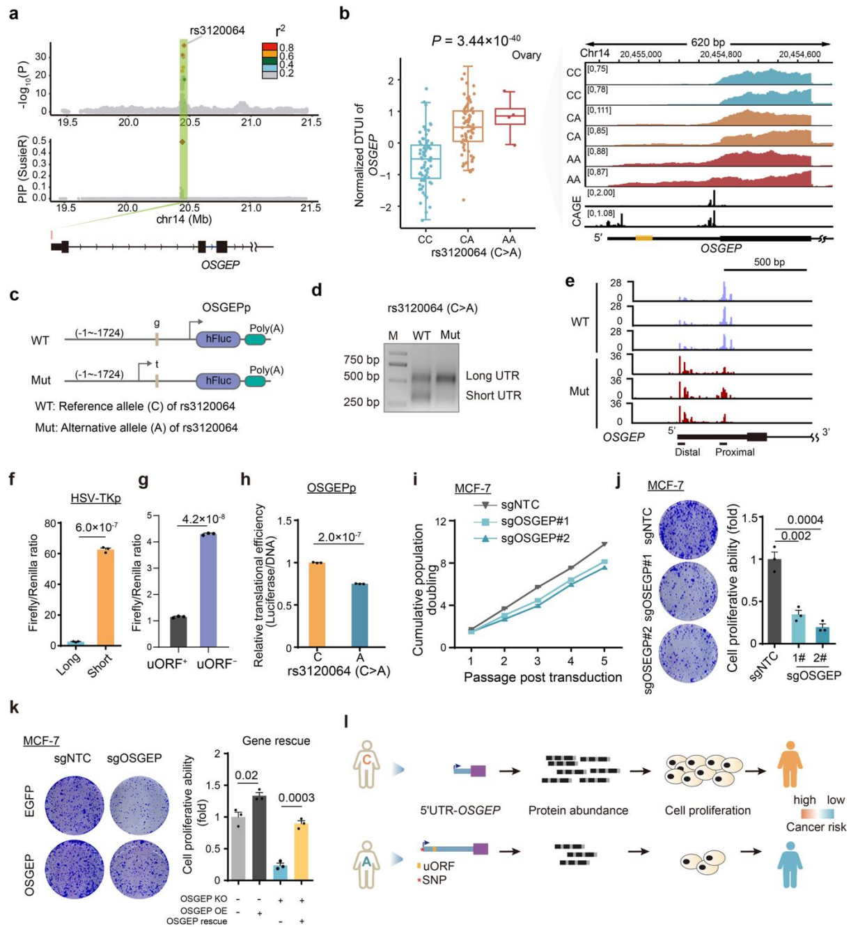
Fig. 6. Alternative TSS regulation of OSGEP is associated with breast cancer risk. a , Regional association plots of the OSGEP gene showing the nominal P values (top) and fine-mapping posterior probabilities (bottom) for the cis -SNPs. b , 5'aVariant (rs3120064) that is strongly associated with the OSGEP 5' UTR usage. Left: Distribution of the normalized DTUI for each genotype. Each dot in the box plot represents the normalized DTUI value for one particular sample. The center horizontal lines within the plot represent the median values and the boxes span from the 25th to the 75th percentile. Right: RNA-seq coverage track for the OSGEP 5' UTR. c , Schematic diagram for the 5'RACE strategy in MCF-7 cells. d , Changes of 5'UTR usage in MCF-7 breast cells detected by 5' RACE. e , Sequencing revealed distal TSS of
